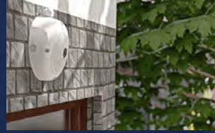
Q26 Hemispheric
