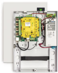
Net2 Entry - Control unit
