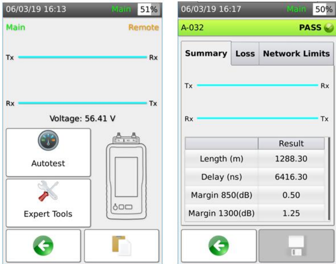
Figure 8: Testing Powered Fibre Cabling
